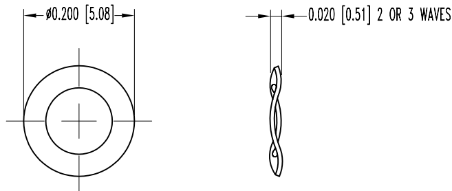
2X WAVE WASHER
