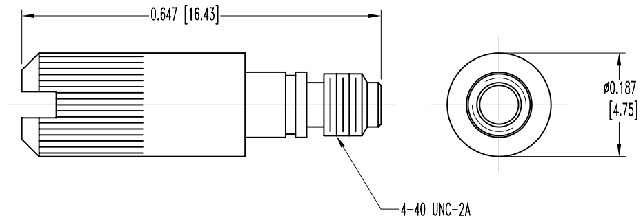
2X THREAD LOCK PILOT
