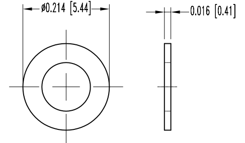
2X FLAT WASHER
