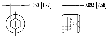
2X SET SCREW
