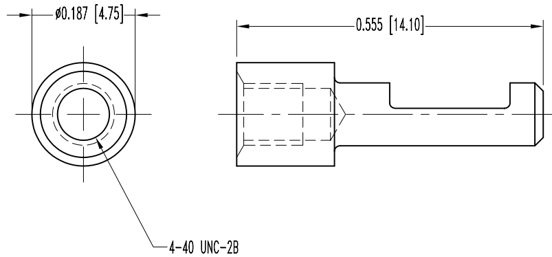
1X FEMALE ROTATING JACKSCREW
