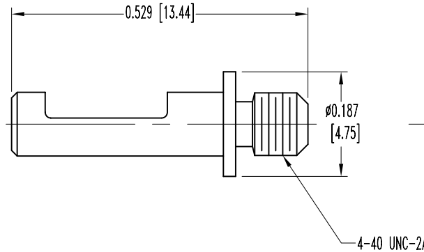
1X MALE ROTATING JACKSCREW
