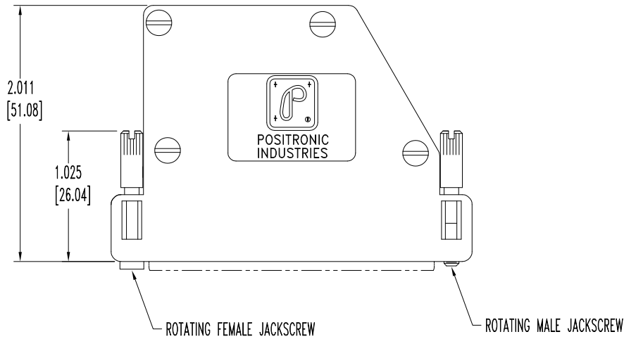
"Y" HOOD
