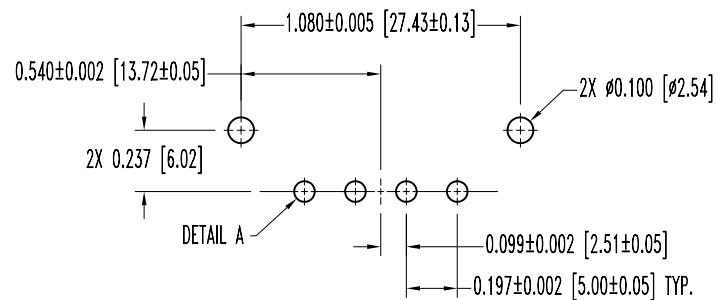
CONTACT HOLE PATTERN
