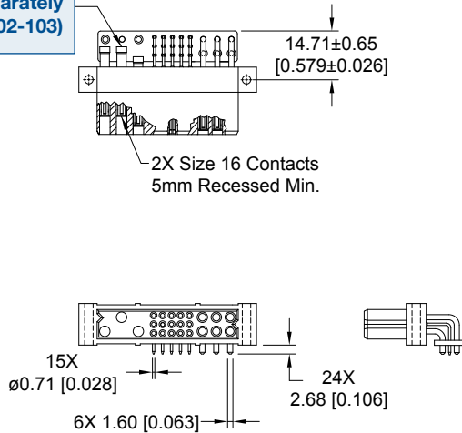
CONNECTOR DIMENSIONS
