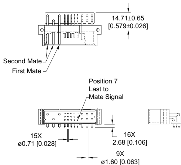
CONNECTOR DIMENSIONS
