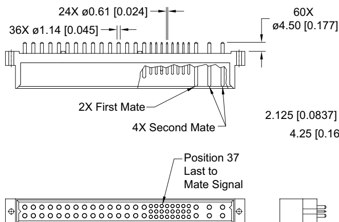
CONNECTOR DIMENSIONS
