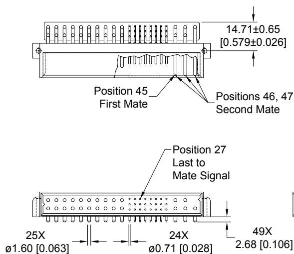
CONNECTOR DIMENSIONS
