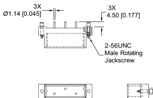
CONNECTOR DIMENSIONS
