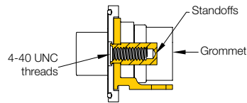
C1 Inside wall mount, integrated angle brackets with 4-40 standoffs, rear grommet, for use with removable contacts
