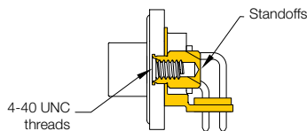
C6 Inside wall mount, 4-40 standoffs, integrated angle brackets, alignment bar, for use with fixed contacts
