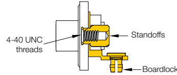
C7 Inside wall mount, integrated angle brackets with boardlocks and 4-40 standoffs, alignment bar, for use with fixed contacts
