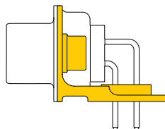
R8 Angle brackets, integrated with shell, 4-40 locknut, alignment bar
