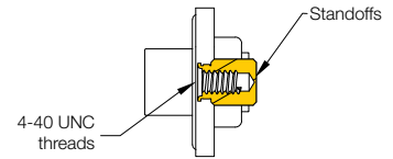
C5 Inside wall mount, 4-40 standoffs
