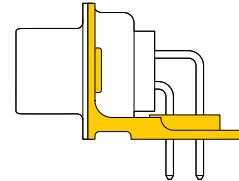
R7 Angle brackets, integrated with shell, 4-40 threaded hole, alignment bar
