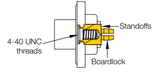
C8 Inside wall mount, 4-40 standoffs with boardlocks, for use with straight PCB termination types
