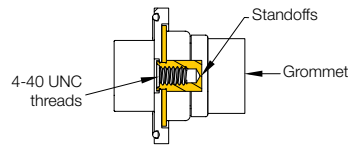
C2 Inside wall mount, 4-40 standoffs, rear grommet, for use with removable contacts
