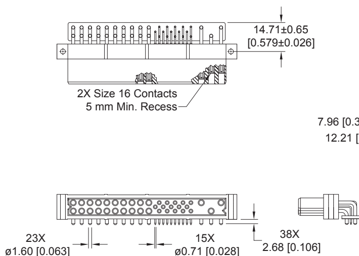
CONNECTOR DIMENSIONS
