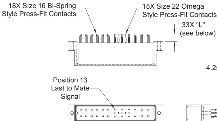
CONNECTOR DIMENSIONS
