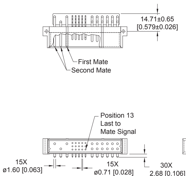
CONNECTOR DIMENSIONS
