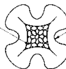
Cross Section of Correctly Crimped Contact
